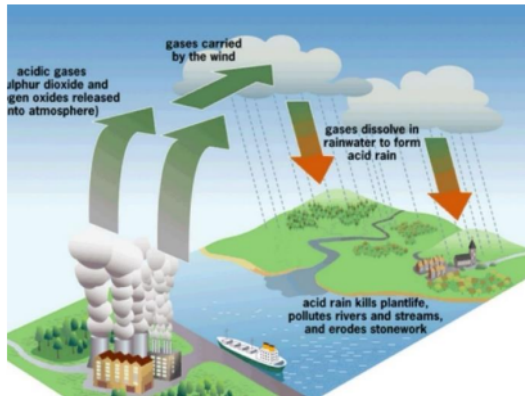
Figure 10: Acid rain
